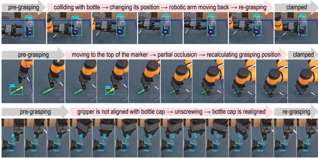
Figure 13: Examples of some interesting findings. Top row : this case comes from the pre-grasping phase of pouring, where the left arm approaches and grasps the bottle. Middle row : this case comes from the pre-grasping phase of inserting, where the right arm approaches and grasps the marker from the top direction. Bottom row : this case comes from the untwisting bottle cap phase of unscrew, where the center of the bottle cap is not aligned with the center point of the end of the gripper. But after a counterclockwise rotation, the upper part of the bottle tilts to the right, and the bottle cap is aligned with the gripper.
